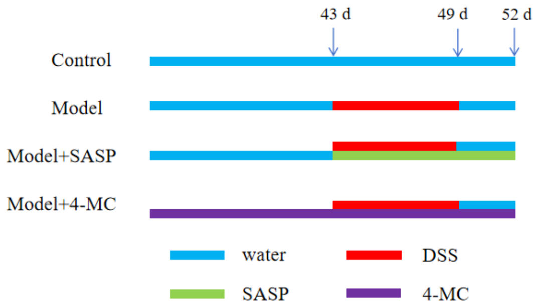
Supplementary Fig. 1. Flow chart of the experimental procedure for this study
